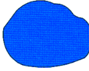
Geoid
