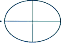
Ellipsoid
