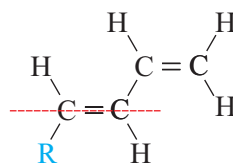
trans -izomer
