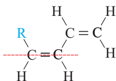
sis -izomer
